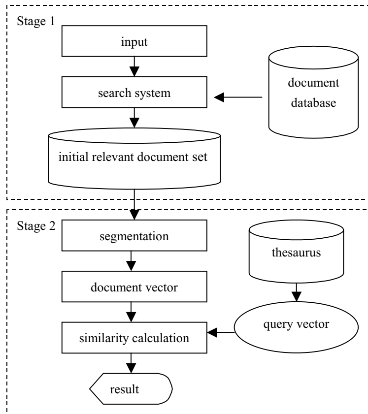
Figure1: system architecture
