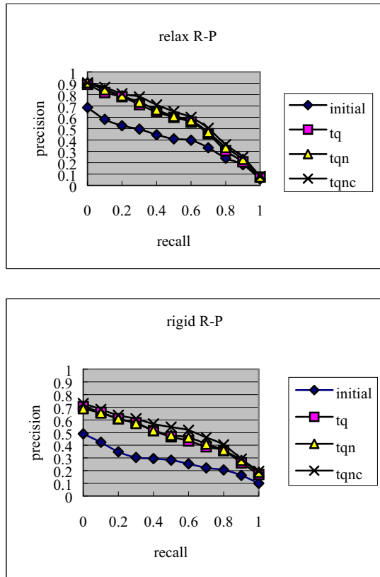
Figure 2: recall-precision curves
